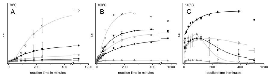
Figure 5. Change in concentration of different aldonic acids during ammoxidation (isobar 0.2 MPa O 2 ) of glucose at 70 °C (A), 100 °C (B), and 140 °C (C). Legend: solid black squares, glycolic acid; open white squares, glycolic acid; solid black circles, tetrionic acid; open white circles, pentonic acid; solid black triangles, hexonic acid. Values for pentonic and hexonic acids are sums of diastereomeric compounds.
