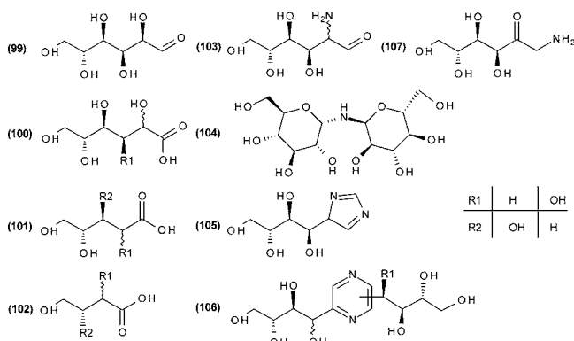
Figure 2. Amoxidation products of glucose with preserved glucose stereoconfiguration.
